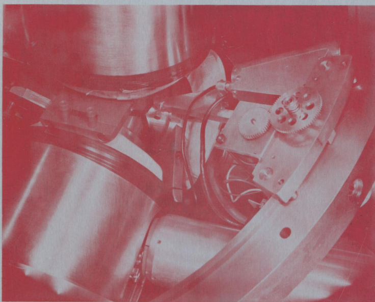
FIG. 5 X-RAY TUBE AND GEARED CARRIAGE DETAIL
